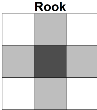
Figure 1: Rook neighbors (light) share an edge with a reference spatial region (dark)[30]
