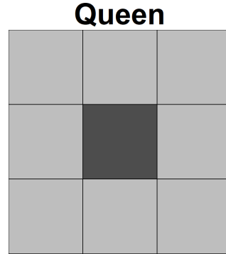
Figure 2: Queen neighbors (light) share either an edge or vertex (or both) with a reference spatial region (dark)[30]
